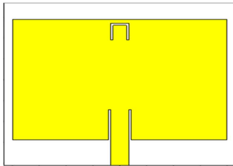
Fig3 Top view of the proposed wearable antenna
