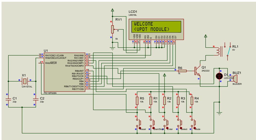
Figure 4: Simulated Circuit diagram of the module
