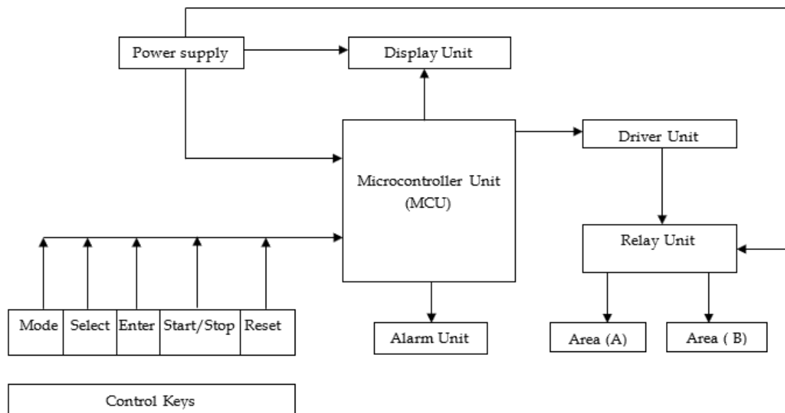
Figure 1. The block diagram of the proposed UPDT switch
