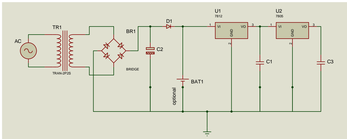
Figure 3: The PSU with a 12 V DC battery option
