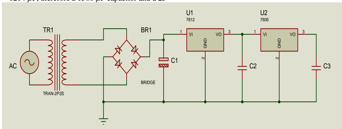
Figure 2: The PSU
