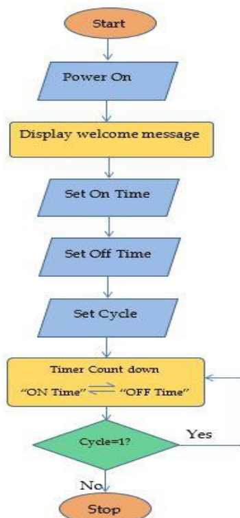
Fig. 6: Flowchart of UPDT Switch
