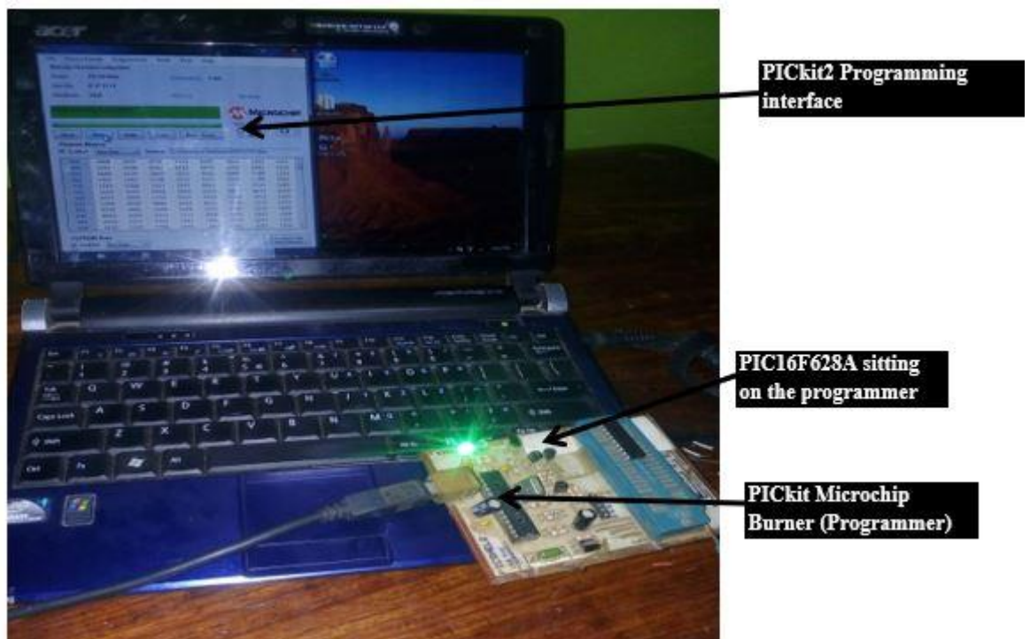
Fig. 5: Software Implementation
